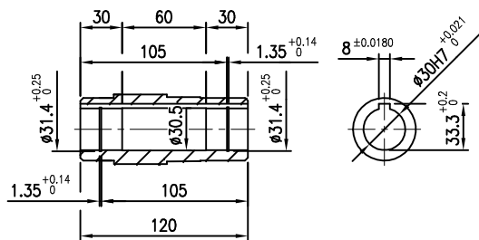
OUTPUT SHAFT(HOLLOW)
